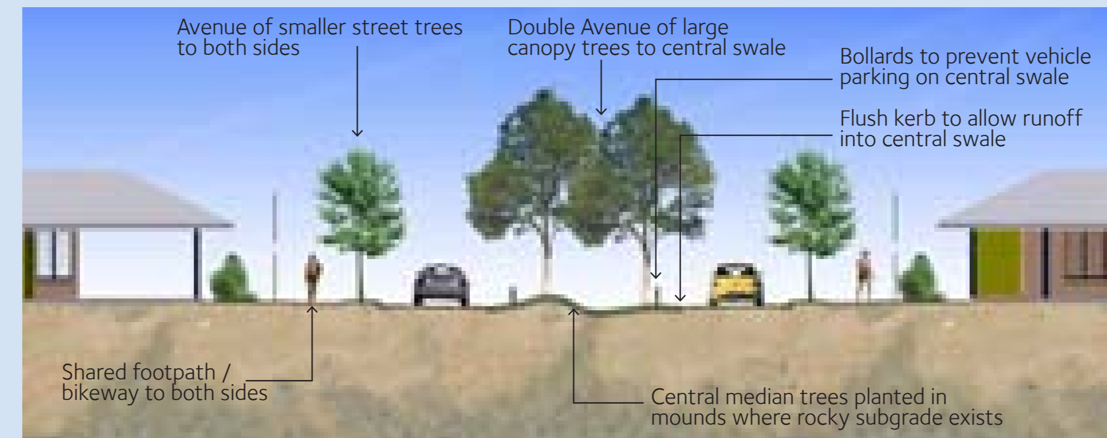
TYPICAL ARRIVAL ROAD OPTION A
