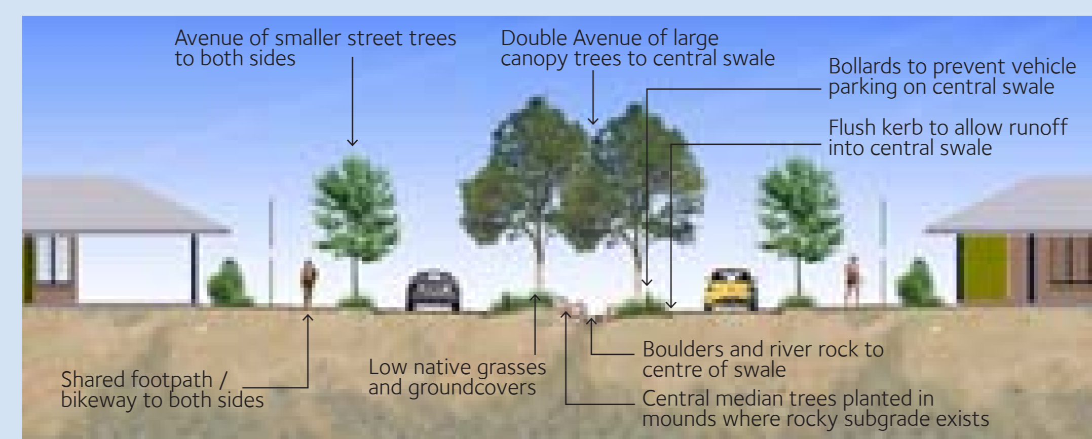
TYPICAL ARRIVAL ROAD OPTION B
